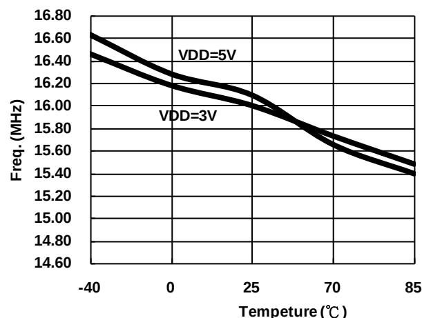
Internal High RC Oscillator (MHz) (Fcpu=IHRC/2~IHRC/16)
