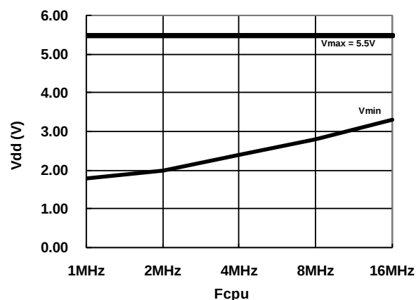
System Minmum Operating Voltage
